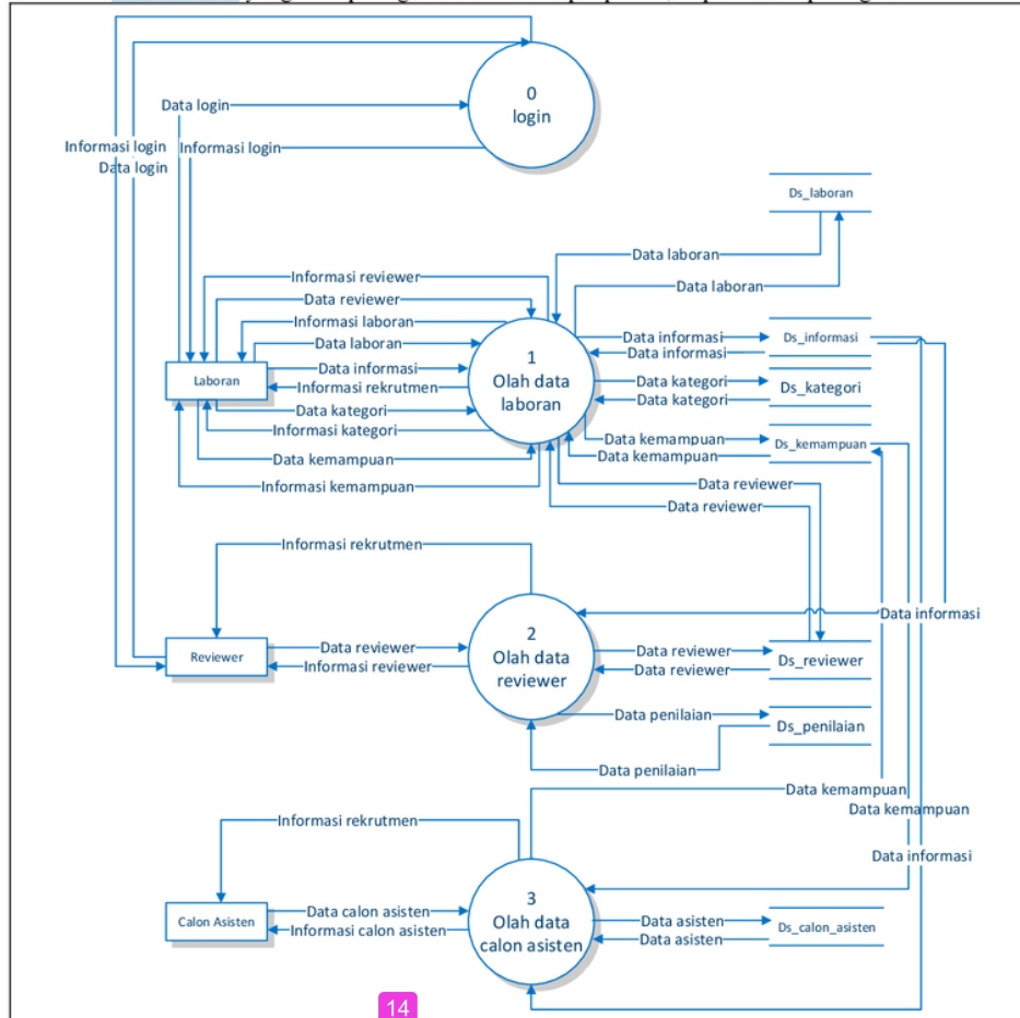
Gambar 4. Data Flow Diagram (DFD) level 1
