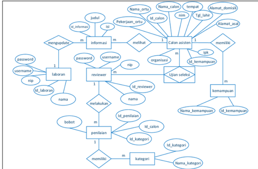
Gambar 1. Entity Relational Diagram (ERD)
