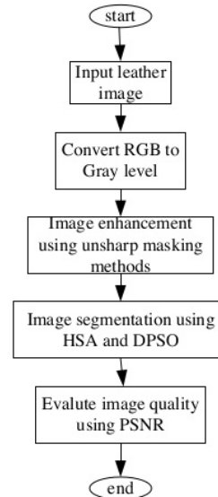
Fig.1 Flow Diagram image segmentation using evolutionary methods
