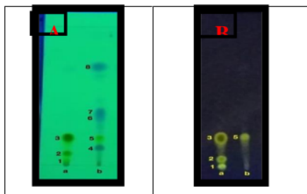
Fig. 1. Thin layer chromatogram profile with the mobile phase of chloroform: dichloromethane in UV 254 nm (A) dan 365 nm (B): a. curcumin standard, b. chloroform extract of bangle.
