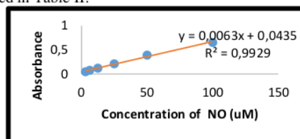
Fig. 2. The standard nitrite curve.
