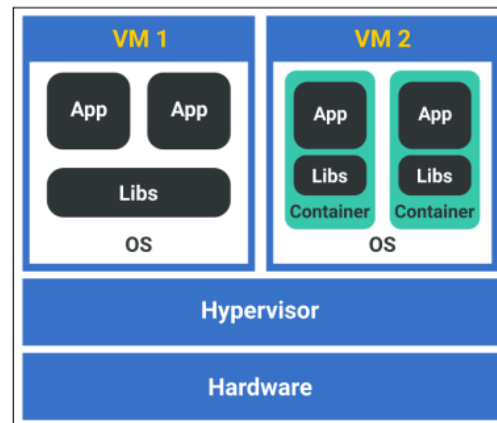
Fig. 2. Comparing various application runtime models.
