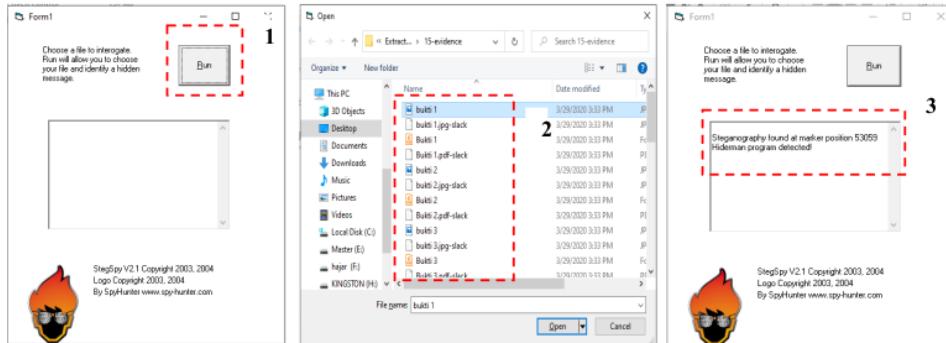
Gambar 12. Proses steganalisis
