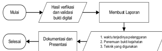
Gambar 4. Flowchart tahap presentation
