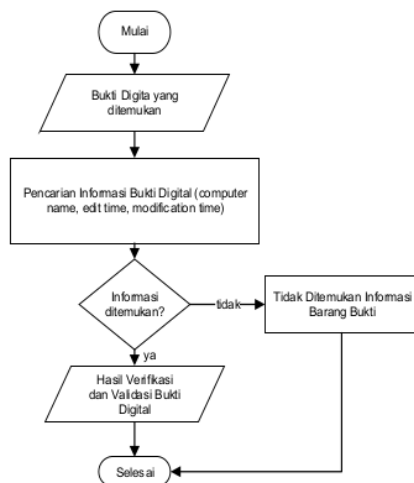
Gambar 4. Flowchart tahap analysis
