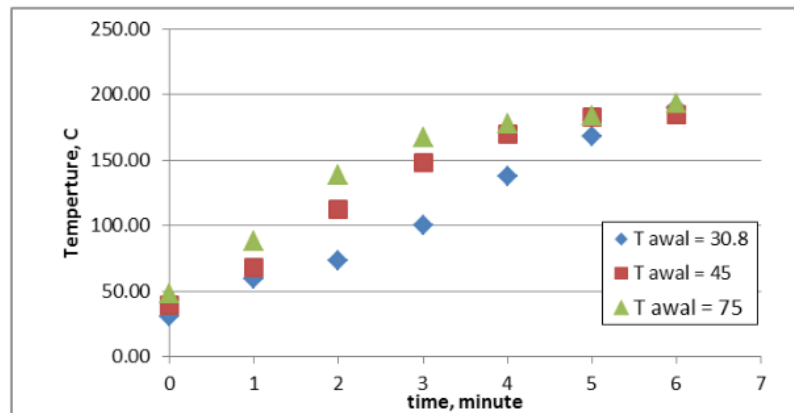
Fig 2. Burning Velocity as function of initial temperature
