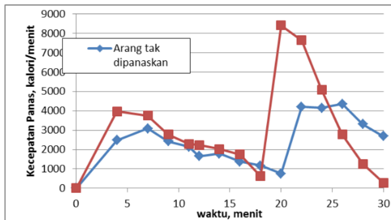
Fig.6. Velocity heat release function of time burning
