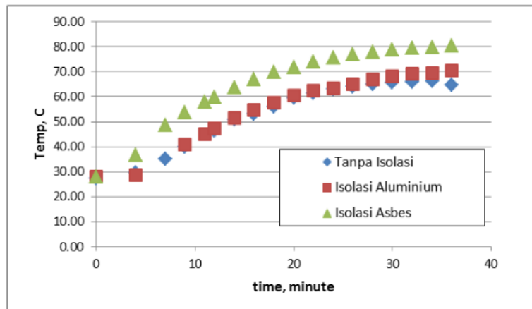
Fig 3. Comparison temperature water
