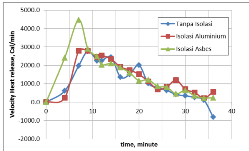
Fig.4. Velocity heat release function of time burning
