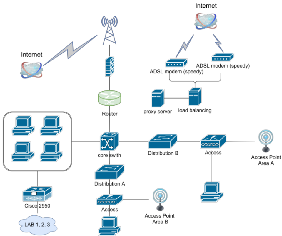
Figure 5. THE PROPOSED STMIK-MPB NETWORK
