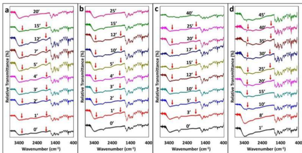
Figure 2. FTIR spectra compilation of DPC from MW treatment: (a) assisted by ethanol, (b) assisted by methanol, (c) assisted by water and (d) neat mixture. Note: red arrows marked the specific peaks of DPC formation.
