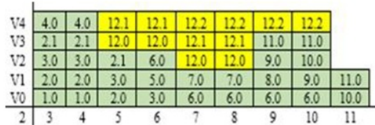
Fig 5. Allocation / parametric jobs (Logical View) planning for reservation requests using FCFS-LRH
