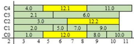
Fig 6. The mapping results on the actual node (Physical View) for parametric jobs
