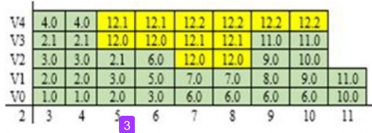
Fig 4. New users have been allocated using FCFS-LRH (Logical View) for parametric jobs.
