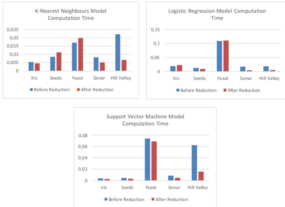
Figure 1. Computational time.
