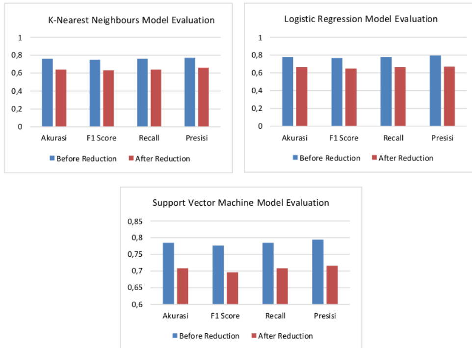
Figure 2. Model Evaluation.
