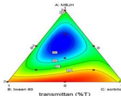
Gambar 1. Contour Plot Transmittan
