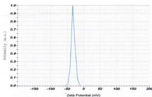
Gambar 4. Zeta potensial droplet SNEDDS MBJH
