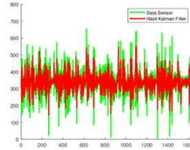
Gambar 5. R=1 Q=1
