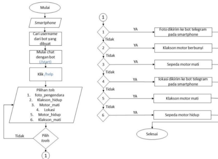
Gambar 6. Flowchart sistem
