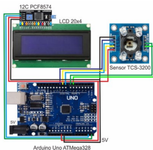
Figure 3. Wiring diagram of glucose level detection system
