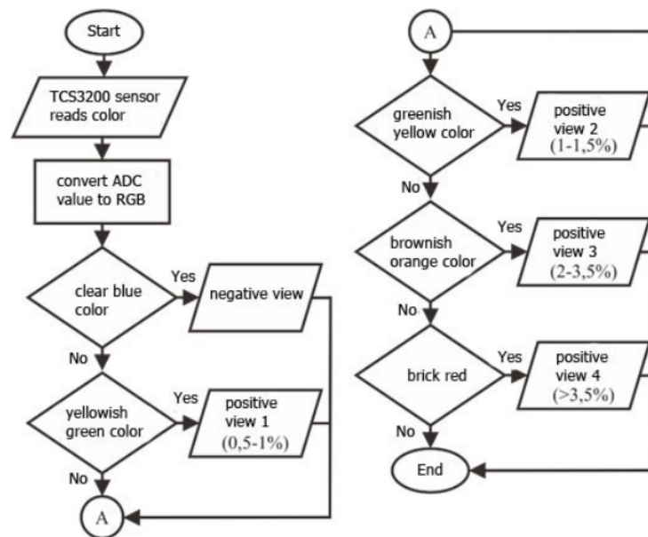
Figure 2. Flowchart of glucose level detection system
