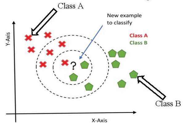
Fig. 2. KNN Visualization
