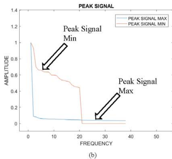
Fig. 7 Average Peak Process (a) Remove Unnecessary Signal and (b) Peak Signal
