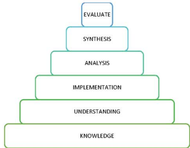
Fig. 8. Bloom Taxonomy
