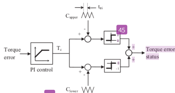
Fig. 6. Constant frequency torque controller (CFTC) [30].
