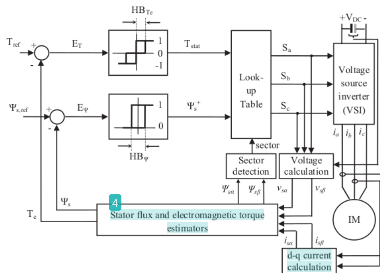
Fig. 1. Control structure of DTC based induction machine.
