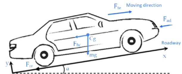
Fig. 10. Elementary forces acting on a vehicle.
