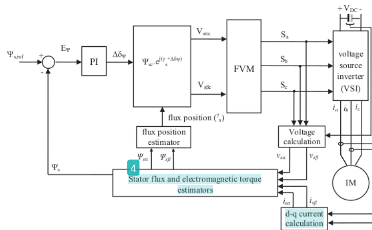
Fig. 5. DTC with voltage FVM.
