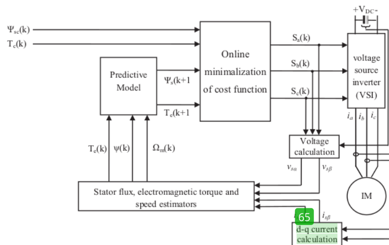
Fig. 8. The simplified block diagram of the DTC-MPC.
