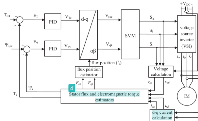
Fig. 4. DTC with voltage SVM.
