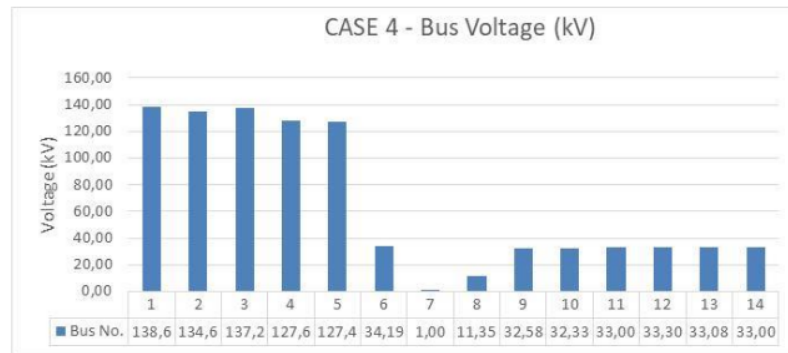
Figure 9. Bus voltage (kV) in case 4
