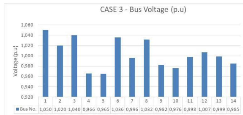
Figure 6. Bus voltage (p.u) in case 3
