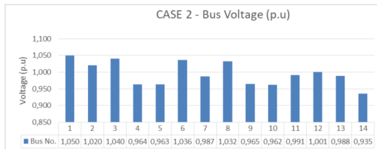
Figure 4. Bus voltage (p.u) in case 2
