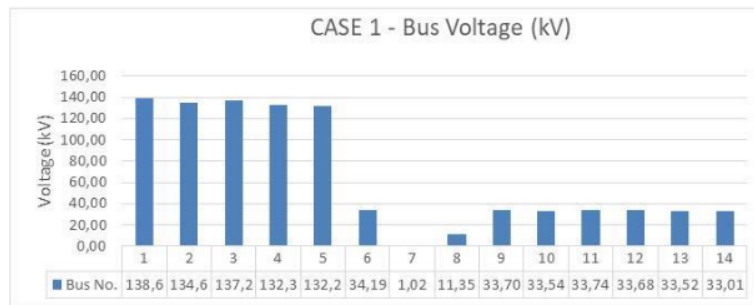
Figure 3. Bus voltage (kV) in case 1
