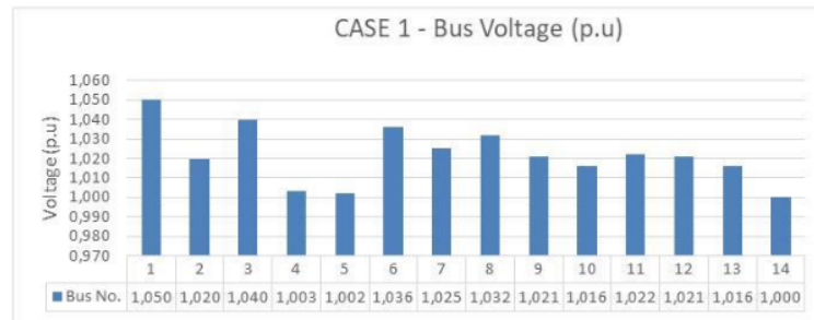
Figure 2. Bus voltage (p.u) in case 1
