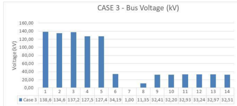
Figure 7. Bus voltage (kV) in case 3
