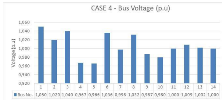
Figure 8. Bus voltage (p.u) in case 4
