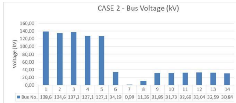
Figure 5. Bus voltage (kV) in case 2
