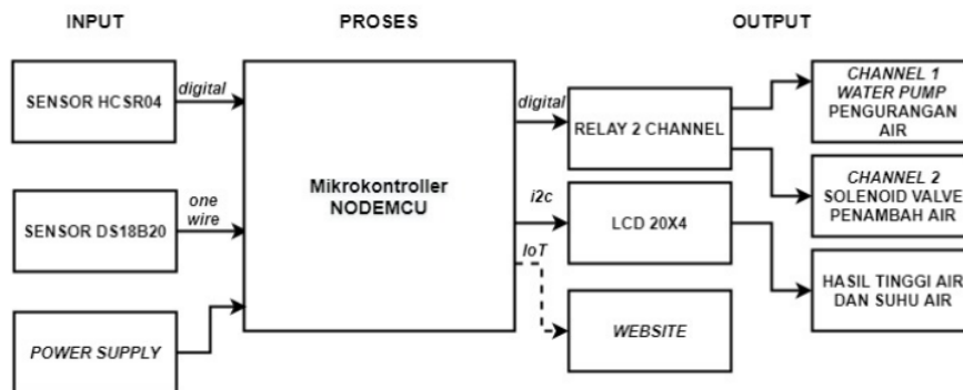
Gambar 1. Diagram Blok
