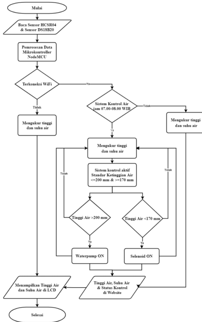
Gambar 2. Diagram Alir
