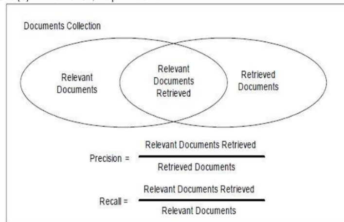
Fig.1. Representation of the Recall Set and Precision [10]
