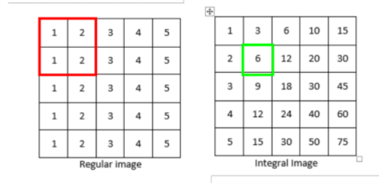
Fig. 2. Example of Integral Image
