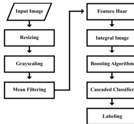
Fig. 4. Research flow
