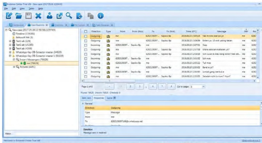
Fig. 9 WhatsApp Key/DB Extractor Message Artifact
