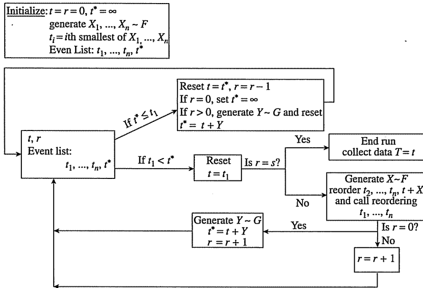
Figure 6.5. Simulating the Repair Model.
