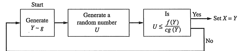
Figure 5.1. The rejection method for simulating a random variable X having density function f .
