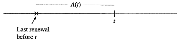
Figure 8.3. Age at t .
