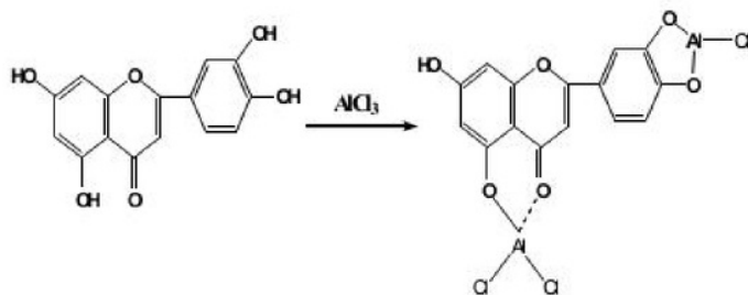
Figure 3. Complex-forming reaction between flavonoid and aluminum
