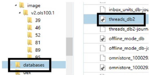
Fig. 9 The database magnet axiom forensics.
