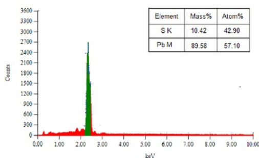
Fig 3. EDX spectrum of PbS thin film.
