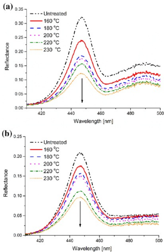
Fig. 2 Reflectance for different heat treatment degrees as a function of wavelength: a horizontal and b vertical grain direction
