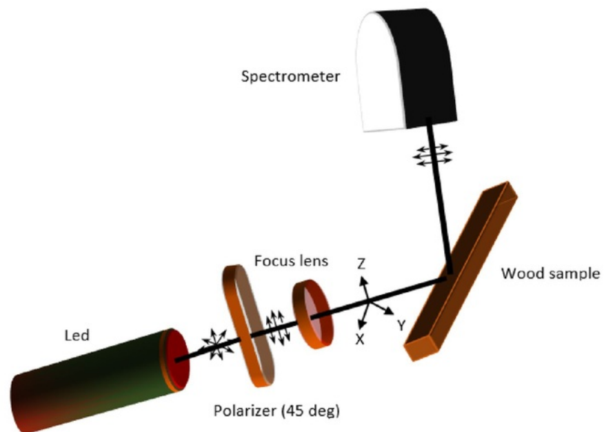
Fig. 1 Schematic illustration of the optical set-up
