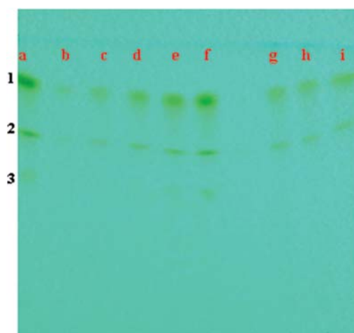
Fig. 1. TLC profile of standard curcumin and temulawak rhizome extract. Legend: spot 1 (Rf 0.78) = curcumin; spot 2 (Rf 0.58) = desmethoxy curcumin; spot 3 (Rf 0.49) = bisdemethoxy curcumin; spot a–f = standard curcumin; and spot g–i = temulawak rhizome extract.
