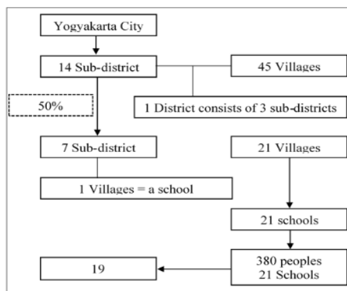
Figure 1: Sampling scheme.
