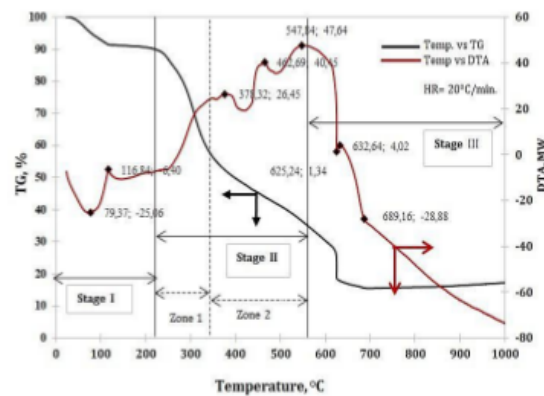
Fig. 3 TG-DTA curve at heating rate: 20°C/min
