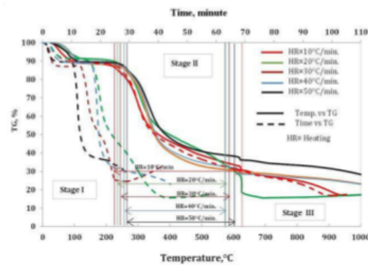
Fig. 2 Thermal decomposition at different heating rates
