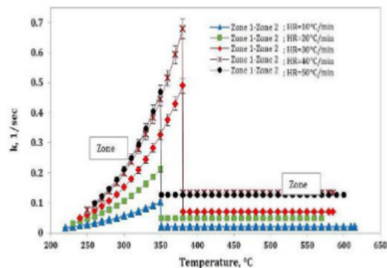
Fig. 9 The relation between the rate of reaction constants (k) and reaction temperature at various heating rates in Zone 1 and Zone 2
