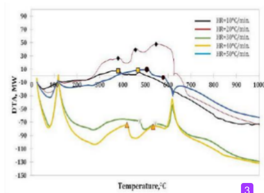
Fig. 4 The peaks on pyrolysis zone of DTA curve at the heating rate of 10, 20, 30, 40 and 50°C/min
