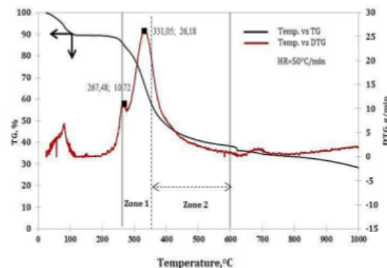
Fig. 5 TG-DTG curve at heating rate 50°C/min
