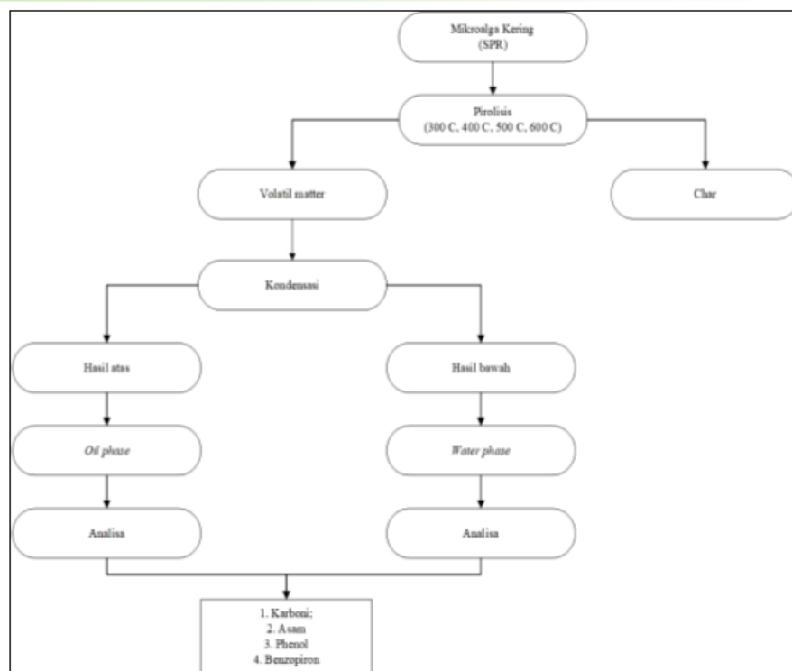
Gambar 2. Prosedur penelitian
