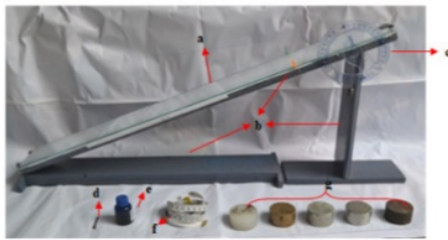
Figure 6. Tools design for determination swipe coefficient on cylinder solid material
