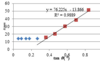
Figure 13. Correlation between \tan \theta and distance of first two-round points ( D ) of stainless steel cylinder.
