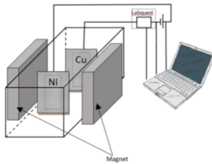
Figure 1. Schematic diagram of the experimental setup
