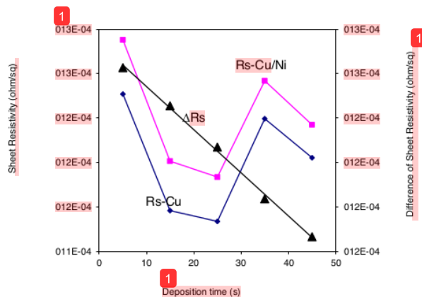
Figure 4. The sheet resistivity of Cu and Cu/Ni
