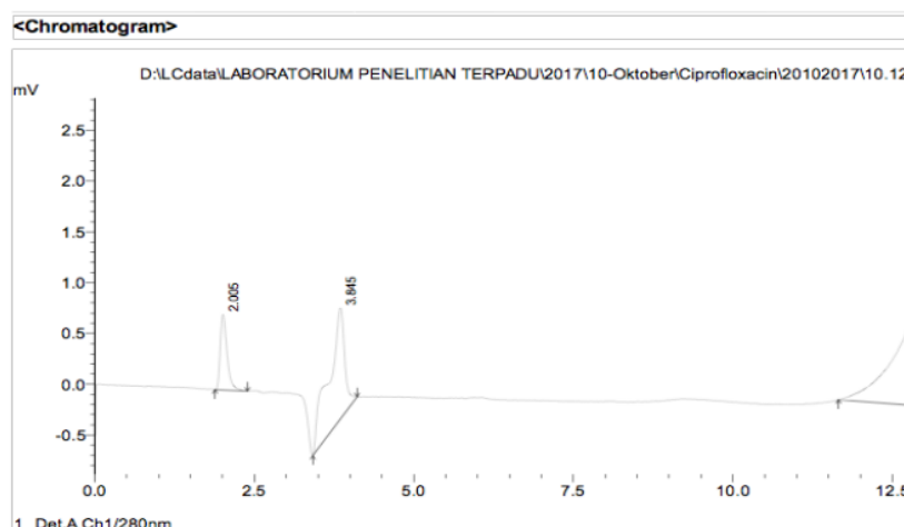
Figure 1: Chromatogram of standard ciprofloxacin
