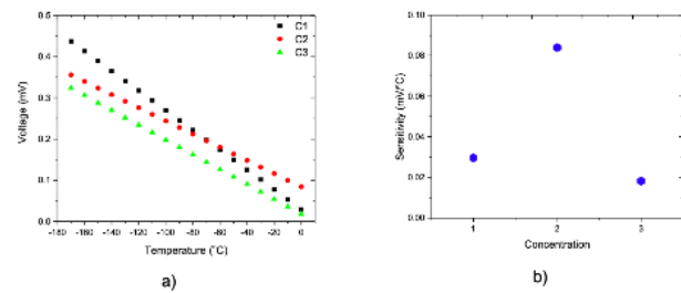
Figure 4. (a). linearity graph and (b) Sensitivity values for Cu/Ni film sensors on changes in liquid nitrogen temperature from -170 °C to 0 °C
