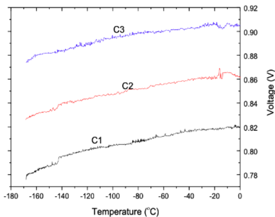
Figure 3. The output voltage and from the Cu/Ni film sample at changes in liquid nitrogen temperature from -170 °C - 0 °C.
