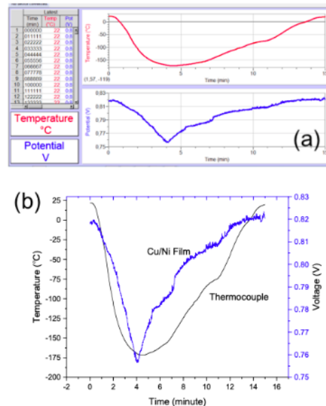
Figure 2. (a). The Data logger pro and (b). Time, voltage and temperature data on sensor performance measurement with voltage output data as data from Cu/Ni film sensors for samples with deposition at concentration 1 (C1)
