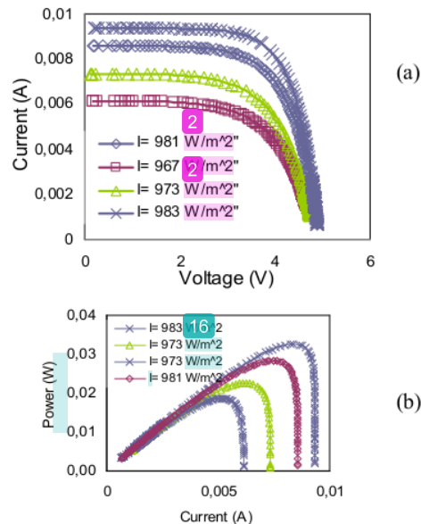
Figure 7. Performance of solar cell on the various intensity. (a) voltage – current curve, (b) Power – current curve
