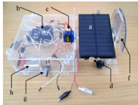
Figure 4. The set of experimental tools, a. Solar cell b. Arduino uno, c. Servo motor, d. Light sensor e. LDR f. Protractor, g. Potentiometer, h. Battery.
