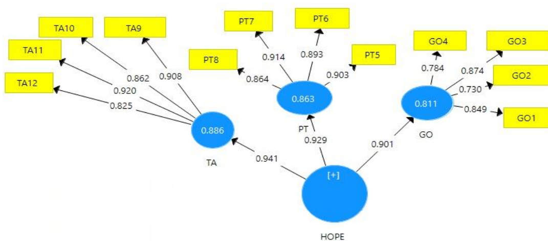
Gambar 1. Output PLS Algorithm Konstruk Hope
