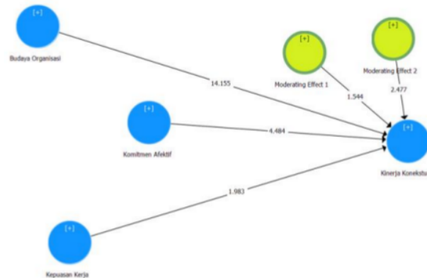
Gambar 1. Path diagram hasil analisis bootstrapping
