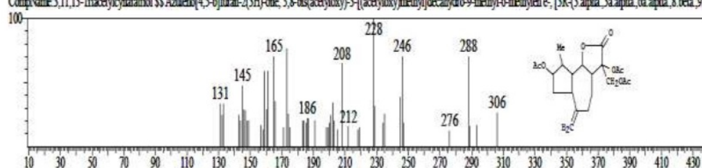
Figure 4. The spectra library of 3,11,13- triacetylcynaratriol (SHIMADZU)
