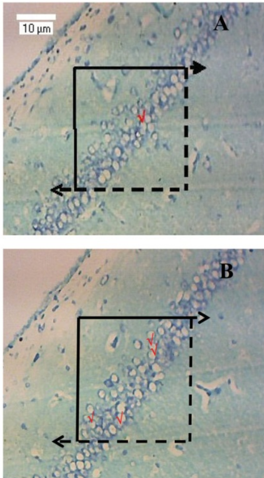
1 Figure 2. (A) and (B) Micrographs from the CA1 pyramidal cell layer of two consecutive sections of 3 μm thickness representing the 'sample section' and 'look-up section' to show the principle of cells counting using physical disector probes. The rectangular frame represents the counting area; broken lines represent the forbidden lines; solid lines represent the inclusion lines. Neurons showing nuclear profiles were used as counting units. The pyramidal cell nuclei, which appear in one section but not in the adjacent section, are marked with red checkmark (✓).
