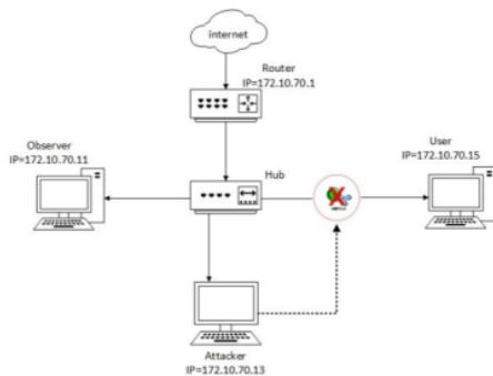
Figure 2. Experiment Scenario of Forensics Analysis
