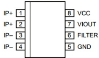
Gambar 2 Pin Out ACS 712
