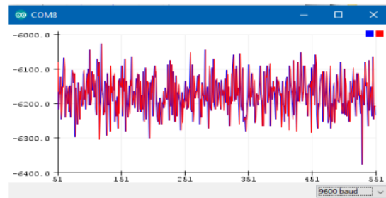
Fig. 3. Accelerometer sensor output x ( Q = 10 , and R = 0.01 )
