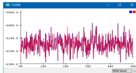
Fig. 6. Gyroscope sensor output x ( Q = 10 , and R = 0.01 )
