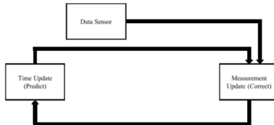
Fig. 5. The Kalman filter algorithm process
