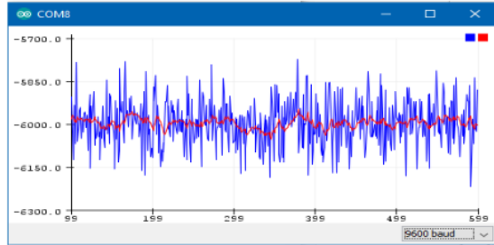
Fig. 13 Gyroscope sensor output x ( Q = 1 , and R = 100 )
