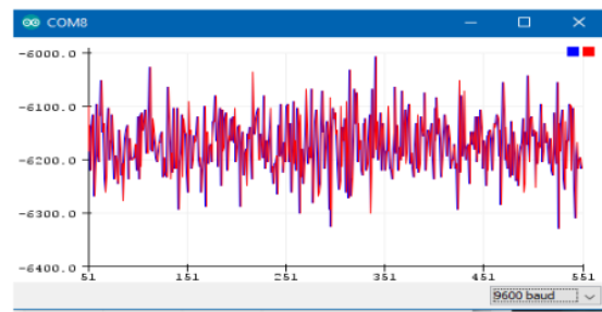
Fig. 2. Accelerometer sensor output x ( Q = 10 , and R = 0.1 )
