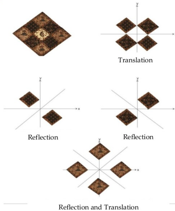
Figure 8. Geometry transformation of Sidowirasat pattern (Risdiyanti & Prahmana, 2020)
