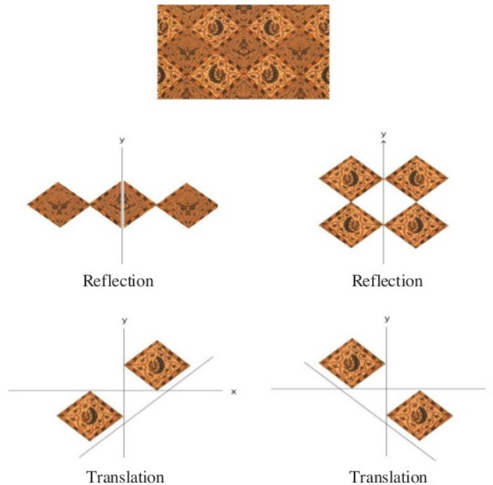
Figure 4. Geometry transformation of Sidomukti pattern (Risdiyanti & Prahmana, 2020)
