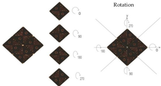
Figure 7. Geometry transformation of Soblog pattern (Risdiyanti & Prahmana, 2020)
