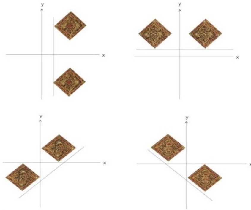
Figure 6. Geometry transformation of Sidoluhur pattern (Risdiyanti & Prahmana, 2020)
