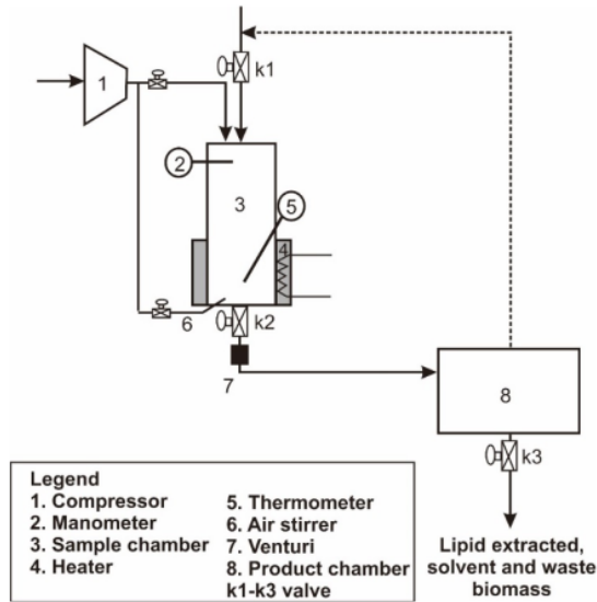
Fig. 2. Hydrodynamic Cavitation Equipment
