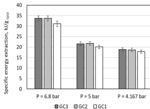
Fig. 4. Effect of cavitation generator geometry and driving pressure on the specific energy of extraction
