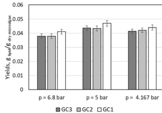
Fig. 3. Effect of cavitation generator geometry and driving pressure on the yields
