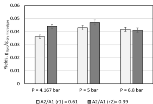
Fig. 5. Effect of the constriction ratio on the extraction yield
