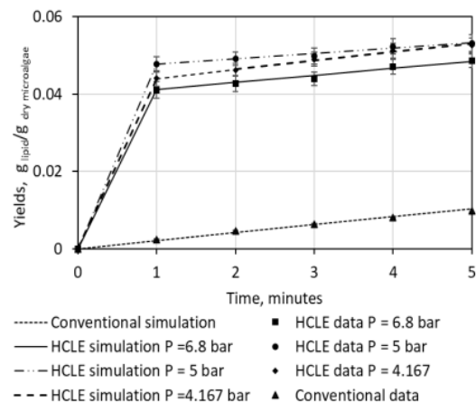
Fig. 6. HCLE and mixing extraction experimental data and simulation result
