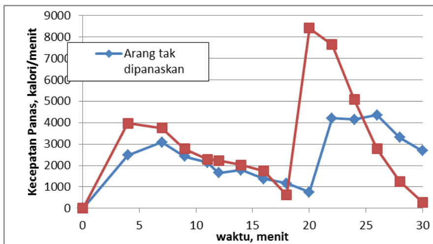
Fig.6. Velocity heat release function of time burning
