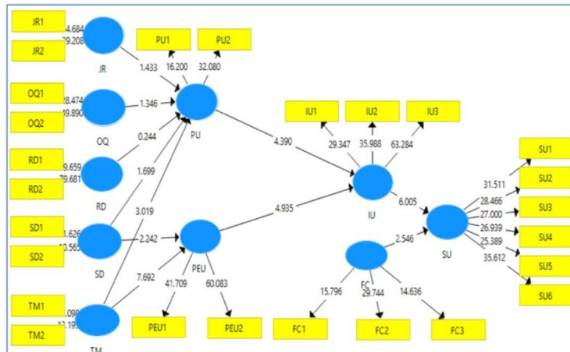
Figure 1. Bootstrapping model result
