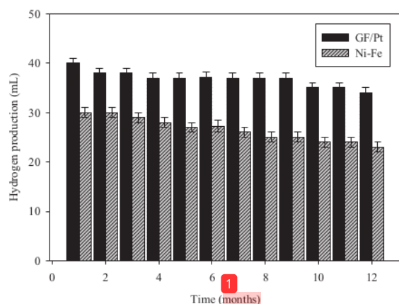
Fig. 6. Trends hydrogen production for twelve months of BES operation.
