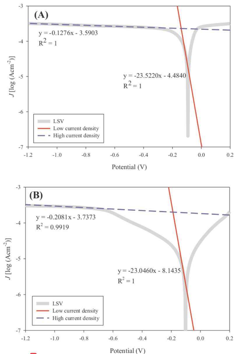
1 Fig. 3. LSV scans with high and low current density for (A) GF/Pt and (B) Ni-Fe.
