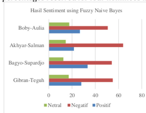
Figure 7. Result of Sentiment using Fuzzy Naïve Bayes
