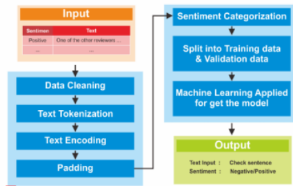
Figure 2. Machine Learning Approach for Sentiment Analysis
