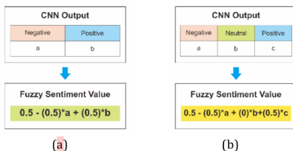
Figure 6. Create Fuzzy Sentiment Value
