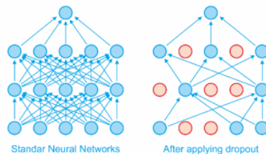
Figure 5. Dropout
