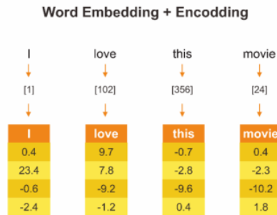
Figure 4. Word Embedding
