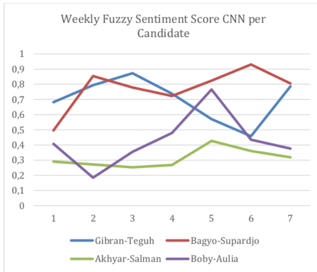
Figure 8. Weekly Fuzzy Sentiment Score CNN per Candidate
