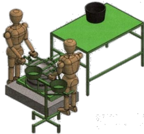
1 Figure 1 The design of the improved wok molding station
