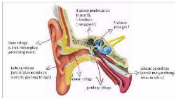
Gambar 11. Anatomi telinga
